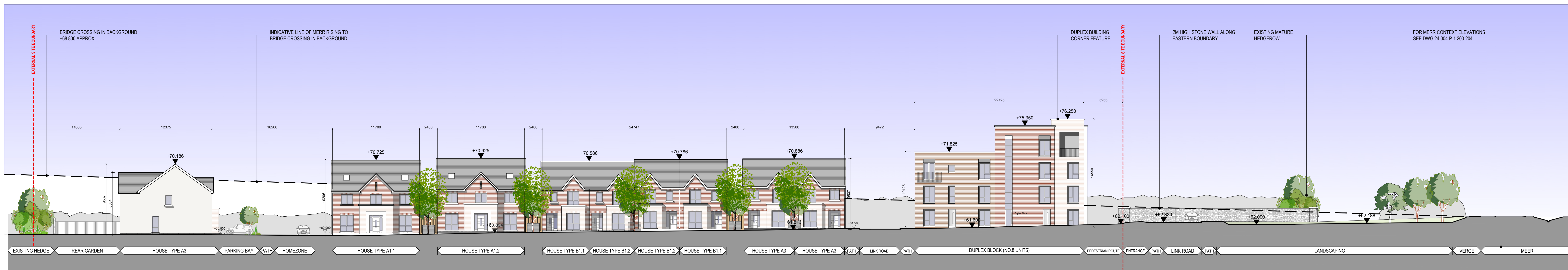
Contiguous Elevation C-C Scale 1:200
